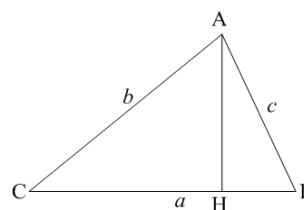
Figure 4 Diagram for Elias Loomis's proof of Heron's Formula.
